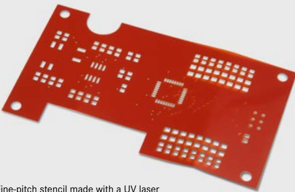
Fine-pitch stencil made with a UV laser for application of solder paste
