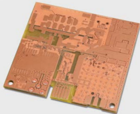
HDI board with ultrafine structures; processing with UV laser and milling/drilling technology
