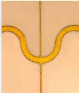
RF structure, Au on Al 2 O 3 ceramic
