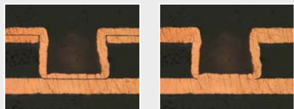
Detached layers from the activation step are reliably eliminated in the via-cleaning step.
